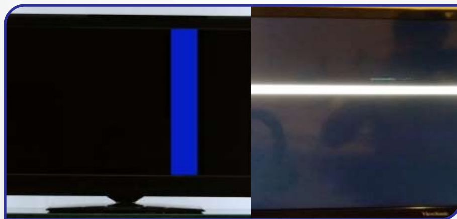
Vertical/Horizontal Bar /Band Panel Repairing
